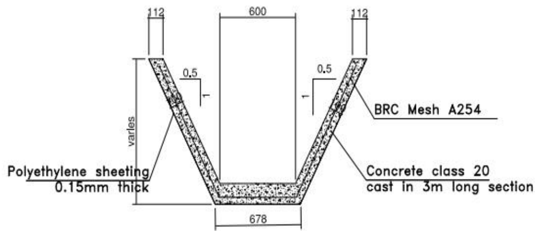
Typical Cross Section: Concrete lined Ditch
